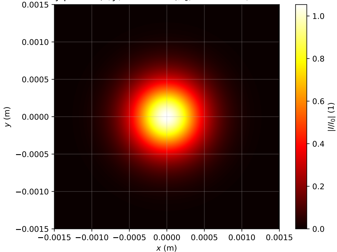
Intensity profile I(x, y, z = 0.955m)/I_0 , P_{in}=0.5P_{cr} , artificial time
